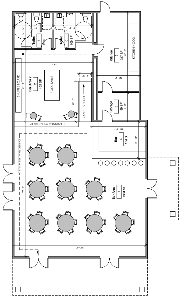
① Floor Plan 3/16" = 1'-0"
